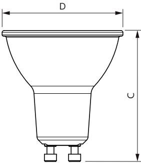
GU10 220-240V 65W 460lm 36D 3000K ND
