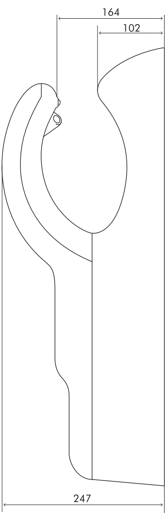
SIDE ELEVATION
