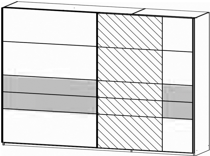
5551 271W X 62D X 210H cm 5544 226W X 62D X 210H cm 5500 181W X 62D X 210H cm
