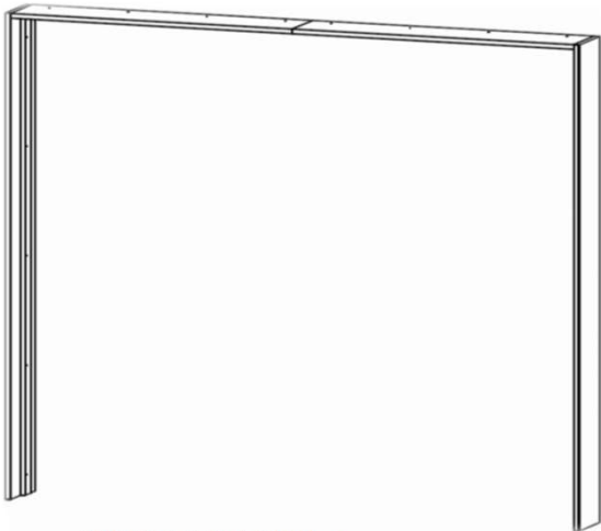
9P4L 278W X 23D X 214H cm 9P3L 233W X 23D X 214H cm 9P2L 189W X 23D X 214H cm
