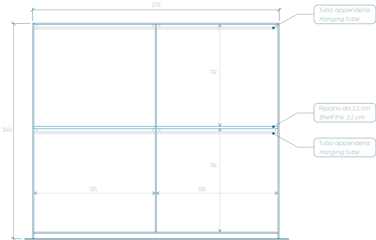
VISTA FRONTALE - FRONT VIEW
