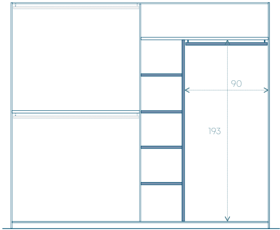
ARMADIO 275 CON TRAMEZZO, RIPIANI E TUBO APPENDERIA WARDROBE 275 WITH VERT. PARTITION, SHELVES AND HANGING TUBE
