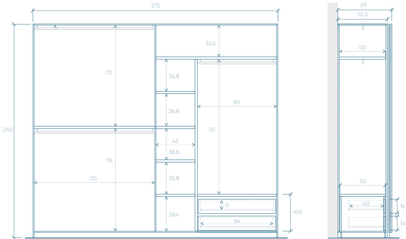
VISTA FRONTALE - FRONT VIEW
